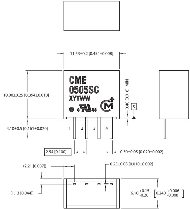
PIN CONNECTIONS - 4 PIN SIP
