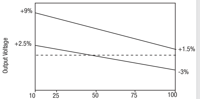
MEU1S0515ZC
