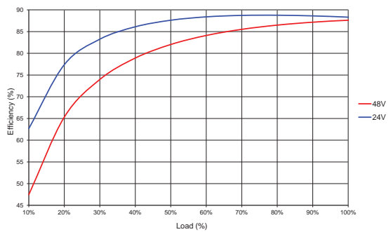
NCS12S4805C
