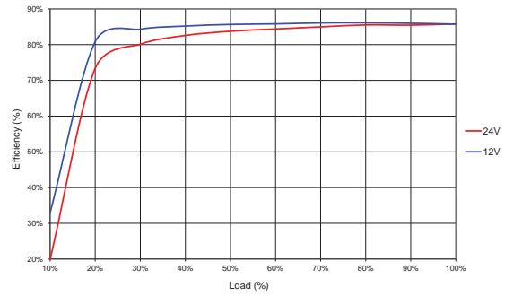
NCS12D4805C
