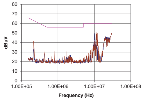
NCS12D1212C
