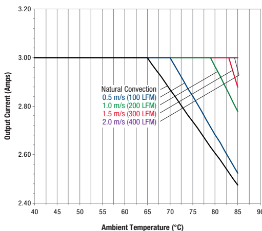
Maximum Current Temperature Derating @sea level ( V_{IN} = 24V , transverse airflow, with baseplate)
