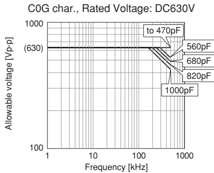
The temperature of the surface of capacitor: 125°C or less (including self-heating)
