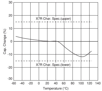
X7R Characteristics
