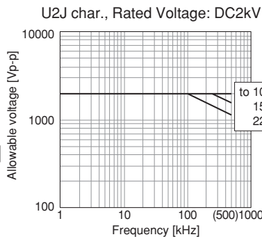
The sine-wave frequency VS allowable voltage
