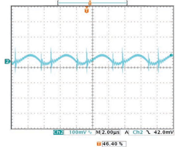
Output Ripple and Noise ( V_{in}=48V , V_{out}=nom , I_{out}=20A , C_{out}=1F \parallel 10\mu F , T_a=+25^\circ C , ScopeBW=20Mhz)
