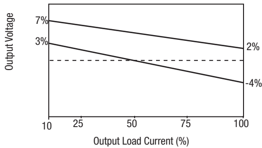
MGJ2D121509SC & MGJ2D241509SC
