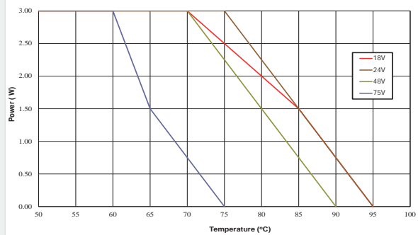
NCS3S4815SC
