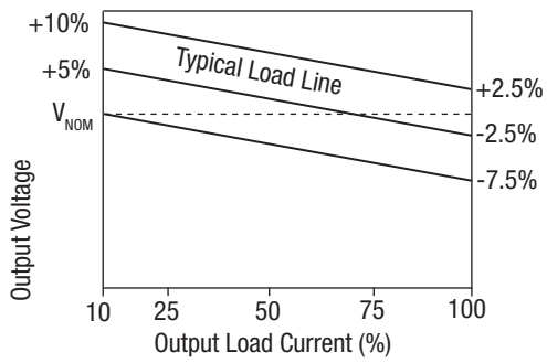
5V, 12V, 15V & 24V Input types
