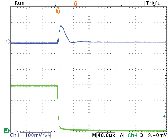
Step Load Transient Response (Vin=7.5V, Vout=5V, Cload=10x10µF X5R 0805 ceramic, plus 1x470µF, 7mΩ POSCAP, total 570µF, Iout=3A to 0A) Top trace=Vout, Bottom trace=Iout
