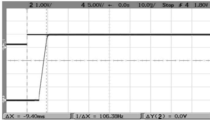
On/Off Enable Startup (Vin=13.8V, Vout=5V, Iout=3A, Cload=0) Trace 4=Enable, Trace2=Vout
