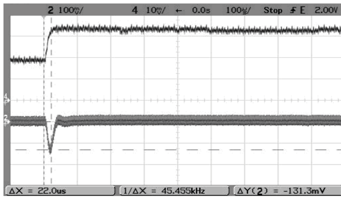
Step Load Transient Response (Vin=12V, Vout=5V, Cload=0, Iout=1.5A to 3A) Trace 2=Vout, Trace 4=Iout, 1A/div.
