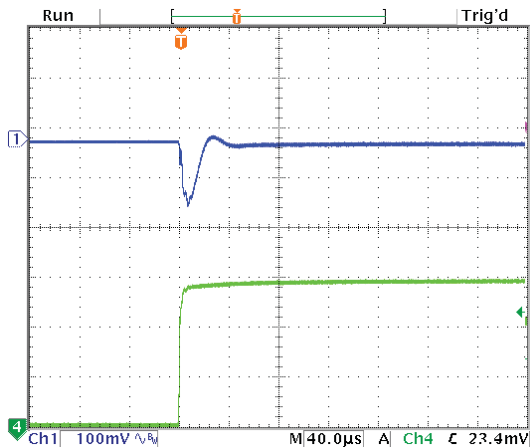
Step Load Transient Response (Vin=5.5V, Vout=3.3V, Cload=10x10µF X5R 0805 ceramic, plus 1x470µF, 7mΩ POSCAP, total 570µF, Iout=0A to 3A) Top trace=Vout, Bottom trace=Iout
