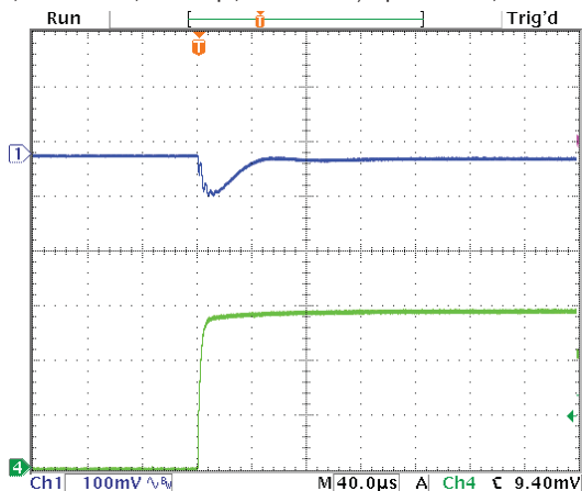
Step Load Transient Response (Vin=12V, Vout=3.3V, Cload=10x10µF X5R 0805 ceramic, plus 1x470µF, 7mΩ POSCAP, total 570µF, Iout=0A to 3A) Top trace=Vout, Bottom trace=Iout
