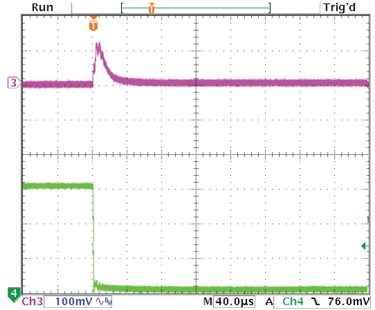
Step Load Transient Response (Vin=7.5V, Vout=5V, Cload=5x10µF X5R 0805 ceramic, total 50µF, Iout=3A to 0A) Top trace=Vout, Bottom trace=Iout
