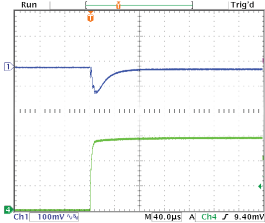
Step Load Transient Response (Vin=7.5V, Vout=5V, Cload=10x10µF X5R 0805 ceramic, plus 1x470µF, 7mΩ POSCAP, total 570µF, Iout=0A to 3A) Top trace=Vout, Bottom trace=Iout
