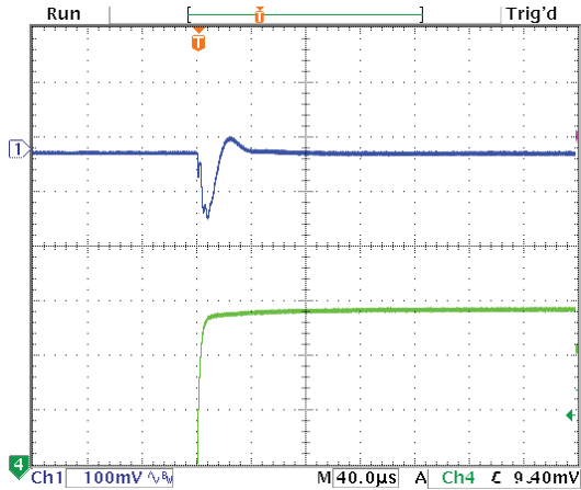
Step Load Transient Response (Vin=12V, Vout=5V, Cload=12x10µF X5R 0805 ceramic, total 120µF, Iout=0A to 3A) Top trace=Vout, Bottom trace=Iout
