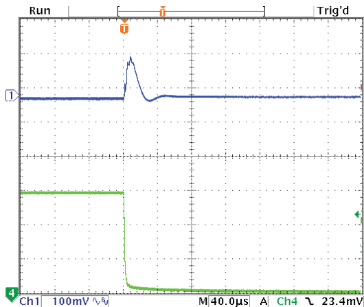
Step Load Transient Response (Vin=5.5V, Vout=3.3V, Cload=10x10µF X5R 0805 ceramic, plus 1x470µF, 7mΩ POSCAP, total 570µF, Iout=3A to 0A) Top trace=Vout, Bottom trace=Iout
