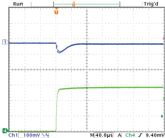
Step Load Transient Response (Vin=12V, Vout=5V, Cload=10x10µF X5R 0805 ceramic, plus 1x470µF, 7mΩ POSCAP, total 570µF, Iout=0A to 3A) Top trace=Vout, Bottom trace=Iout
