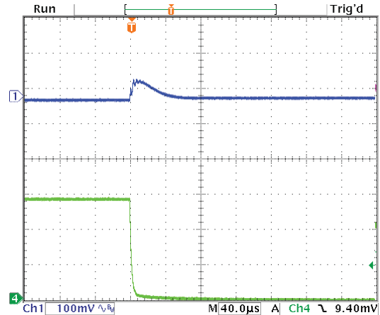
Step Load Transient Response (Vin=12V, Vout=5V, Cload=10x10µF X5R 0805 ceramic, plus 1x470µF, 7mΩ POSCAP, total 570µF, Iout=3A to 0A) Top trace=Vout, Bottom trace=Iout
