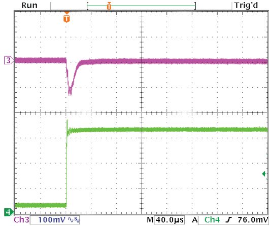
Step Load Transient Response (Vin=7.5V, Vout=5V, Cload=5x10µF X5R 0805 ceramic, total 50µF, Iout=0A to 3A) Top trace=Vout, Bottom trace=Iout
