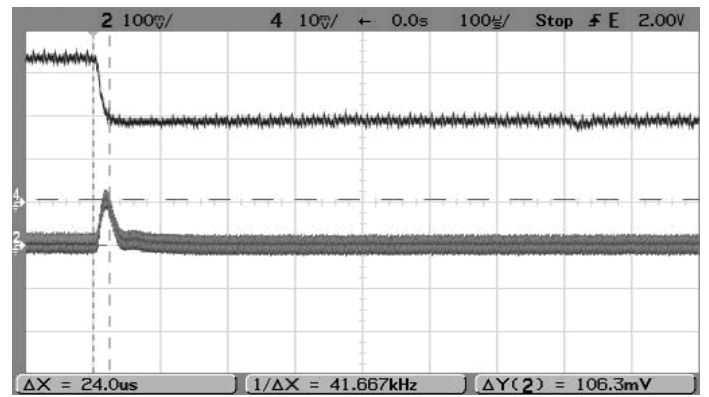
Step Load Transient Response (Vin=12V, Vout=5V, Cload=0, Iout=3A to 1.5A) Trace 2=Vout, Trace 4=Iout, 1A/div.
