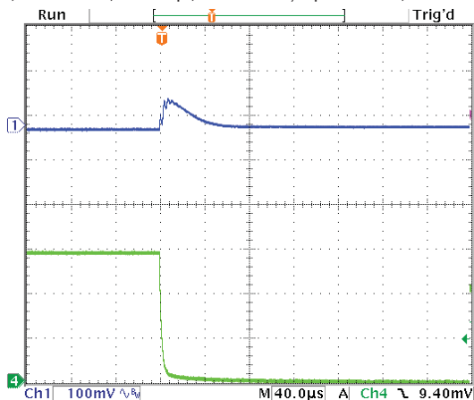
Step Load Transient Response (Vin=12V, Vout=3.3V, Cload=10x10µF 5R 0805 ceramic, plus 1x470µF, 7mΩ POSCAP, total 570µF, Iout=3A to 0A) Top trace=Vout, Bottom trace=Iout
