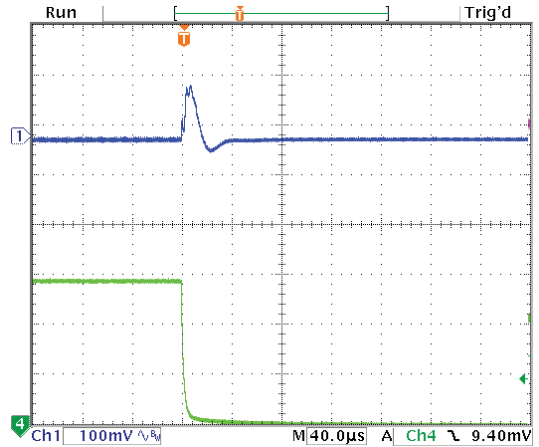
Step Load Transient Response (Vin=12V, Vout=5V, Cload=12x10µF X5R 0805 ceramic, total 120µF, Iout=3A to 0A) Top trace=Vout, Bottom trace=Iout
