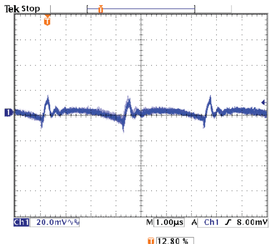
OKX2-T/16-D12 Output Ripple and Noise (V in =12V, V out =0.75V, I out =16A, C in =1000µF, C load =1µF // 10µF, ScopeBW=100MHz)
