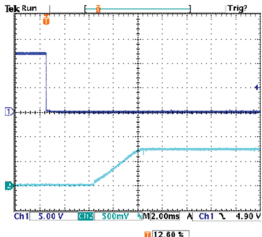
OKX2-T/16-D12-C On/Off Enable Startup Delay (V in =12V, V out =0.75V, I out =16A, C in =1000µF, C load =1µF // 10µF) Trace 1=Enable In, Trace 2=Vout
