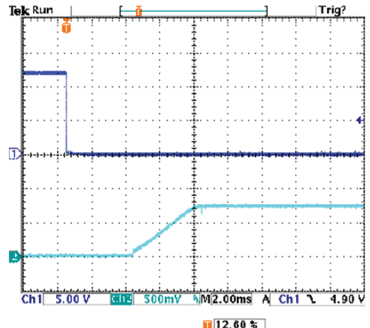
OKX2-T/16-D12-C On/Off Enable Startup Delay (V in =12V, V out =0.75V, I out =16A, C in =1000μF, Load=1μF // 10μF) Trace 1=Enable In, Trace 2=Vout
