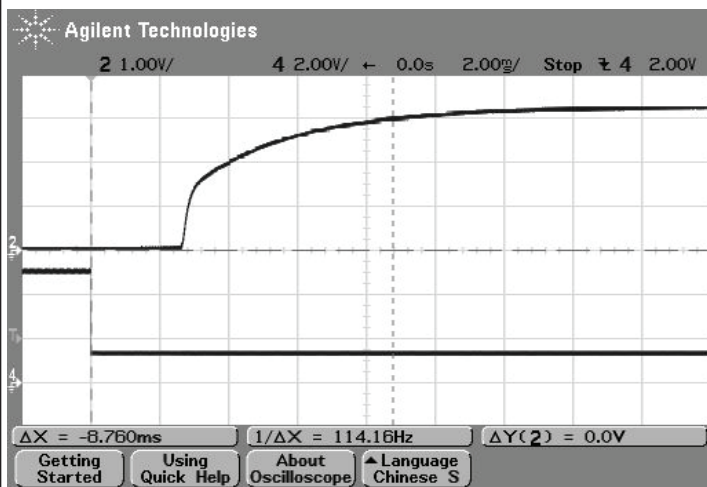
On/Off Enable Delay (Vin=48V, Vout=nom., Iout=25A, Clod=10uF, Ta=+25° C., ScopeBW=20Mhz, Trace 2=Vout, Trace 4=Enable.)
