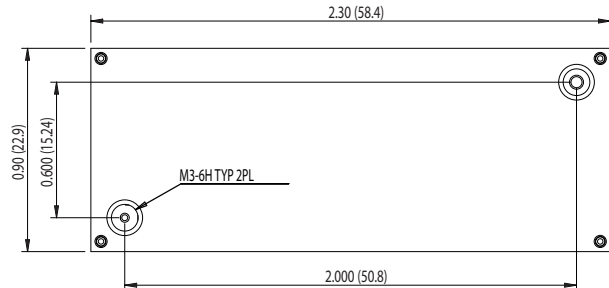
WITH BASEPLATE OPTION
