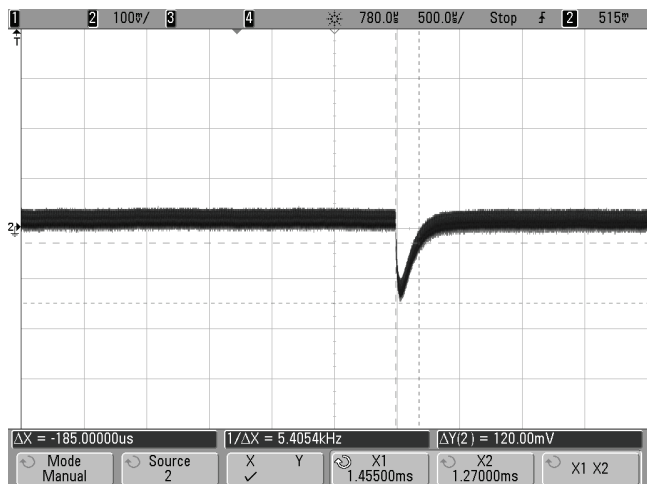
Step Load Transient Response (Vin=48V, Vout=nominal, Cloud=0, Iout=50% to 75% of full load, Ta=+25°C.) Trace 1=Vout, 100 mV/div., 500 μS/div.
