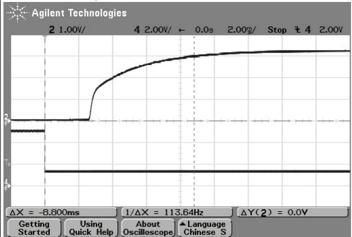
On/Off Enable Delay (Vin=48V, Vout=nom., Iout=30A, Cloud=10uF, Ta=+25° C., ScopeBW=20Mhz, Trace 2=Vout, Trace 4=Enable).
