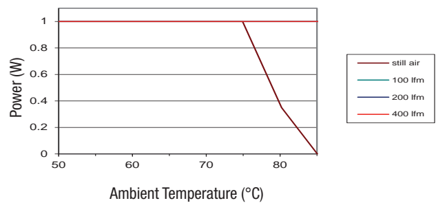
NXJ1S1215MC
