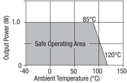
TEMPERATURE DERATING GRAPH - All other types 1
