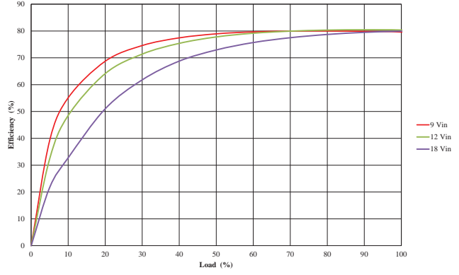
MTC2S1205MC
