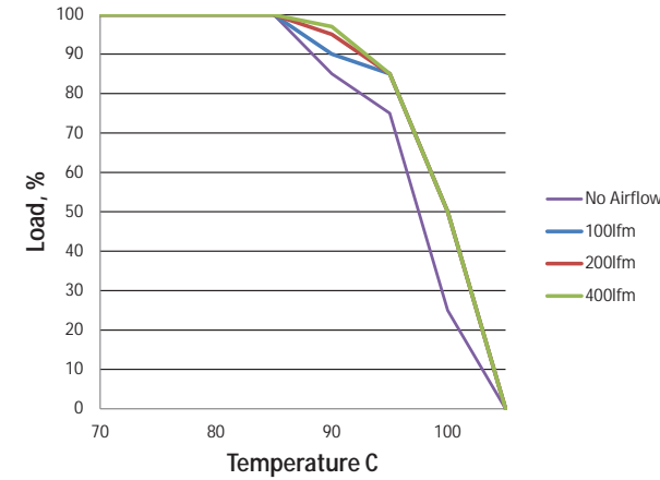
MTC2S2412MC - 36Vin
