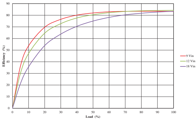
MTC2S1212MC
