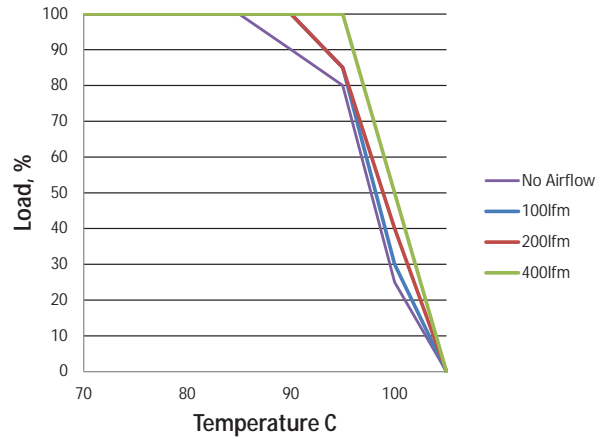
MTC2S1205MC - 18Vin
