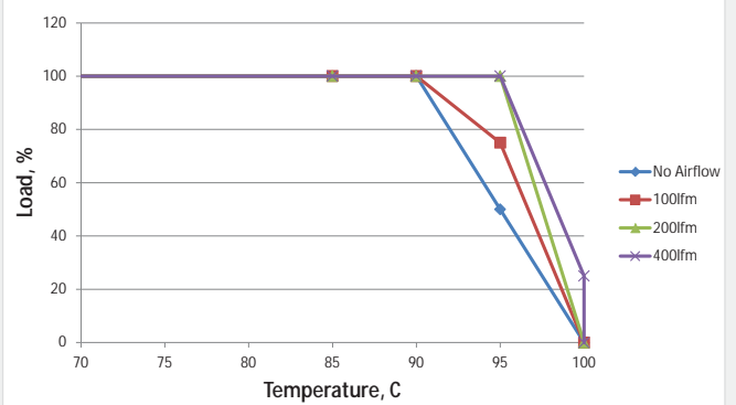
MTC1S2403MC - 18Vin
