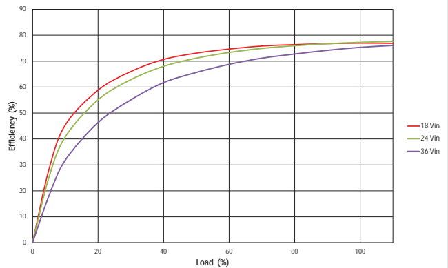
MTC1S2412MC
