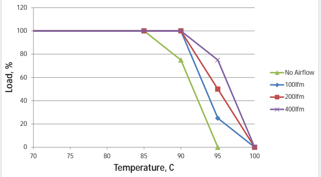
MTC1S1205MC - 18Vin
