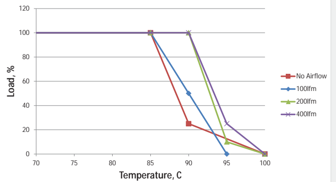
MTC1S2403MC- 24Vin
