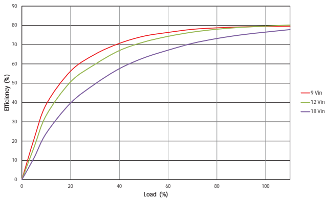
MTC1S1212MC
