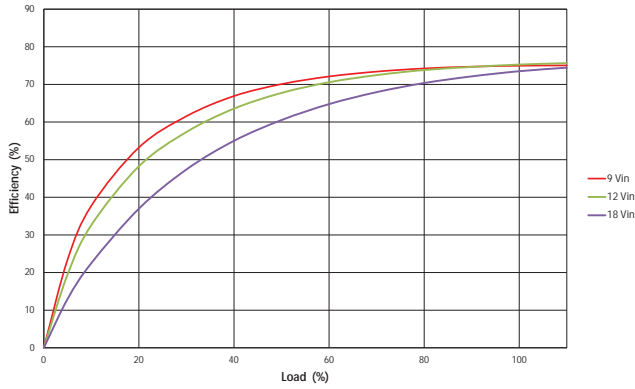
MTC1S1203MC
