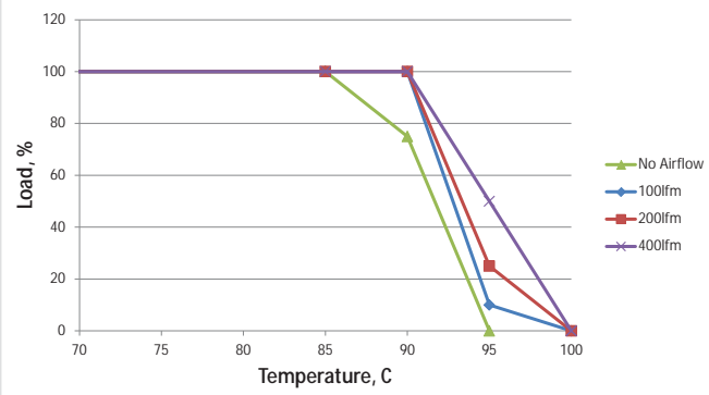
MTC1S2405MC - 36Vin
