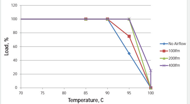
MTC1S2403MC - 18Vin
