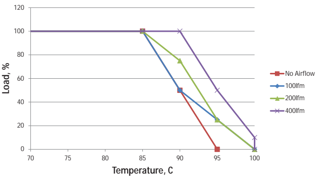
MTC1S1212MC- 12Vin
