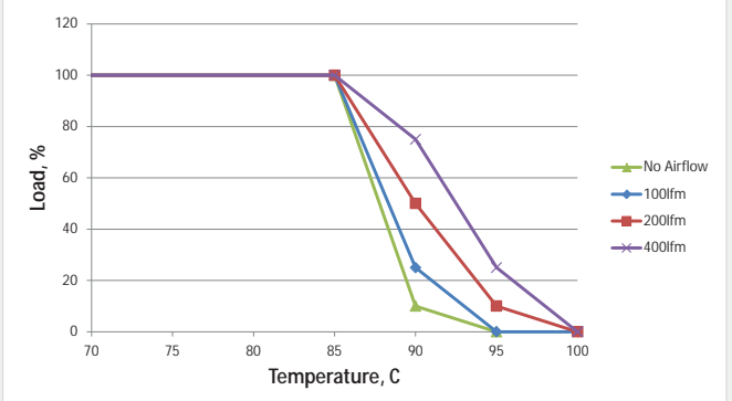
MTC1S2412MC - 36Vin
