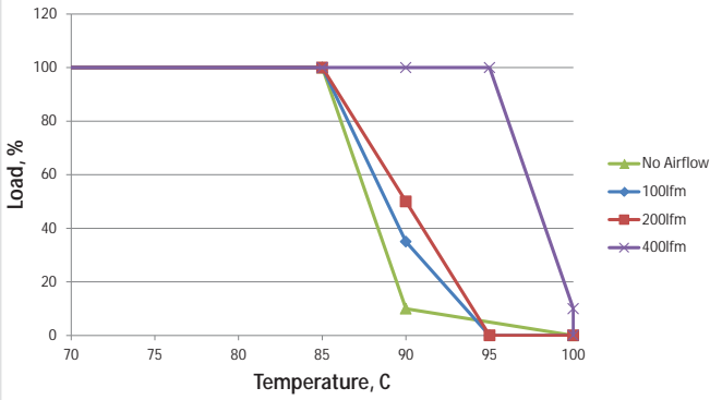
MTC1S1203MC - 18Vin
