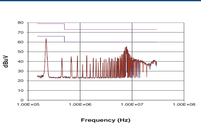
MTC1S2405MC
