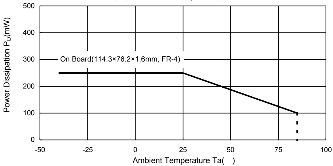
NJU7747/48F4 Power Dissipation ( T_{opr} = -40 \sim +85 , T_j = 125 )
