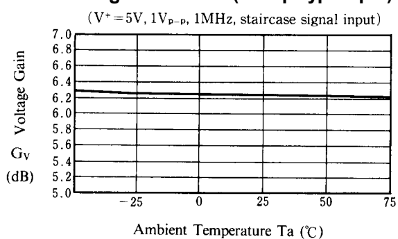
Voltage Gain vs. Ta (Clamp Type Input)
