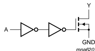
Fig 3. Logic diagram
