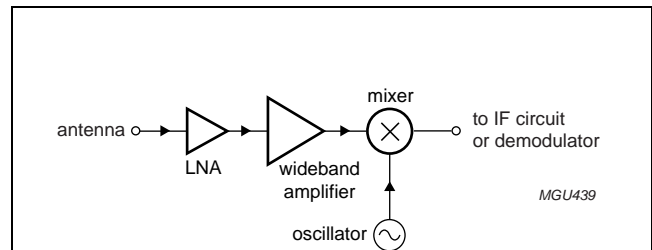
Fig.5 Application as RF amplifier.
