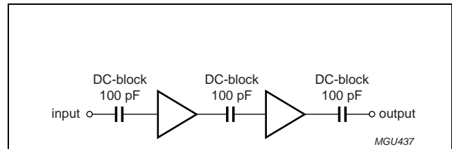
Fig.3 Easy cascading application circuit.
