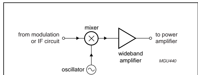
Fig.6 Application as driver amplifier.
