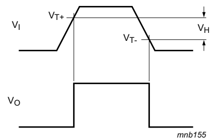
Fig 6. Definitions of V_{T+} , V_{T-} and V_H
