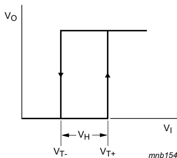
Fig 5. Transfer characteristic
