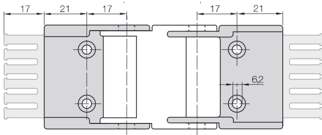
Mounting Brackets, with tie-wrap plates, locking Part. No. 10X.12PZ
