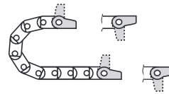
Mounting Brackets, with tie-wrap plates, locking Part. No. 10X.12PZ
