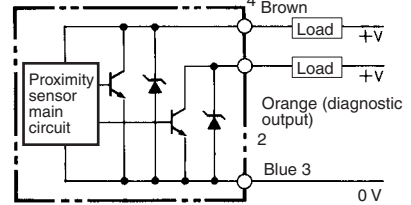
E2E-X□D1S With Diagnostic Output
