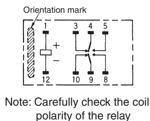
Terminal Arrangement/ Internal Connections (Bottom View)
