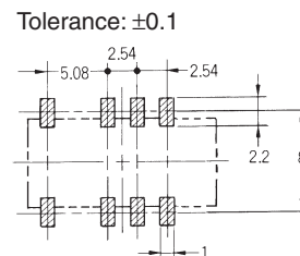
Footprint (Top View)
