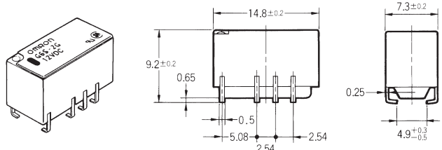
Terminal Arrangement/ Internal Connections (Top View)
