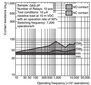
Contact Reliability Test - G6S-2F(G) (Contact Resistance) *1, *2
