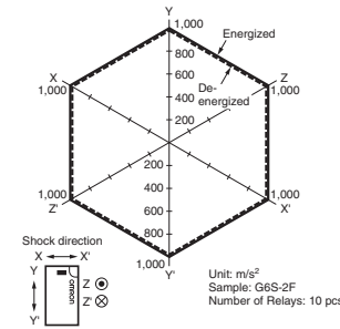
Shock Malfunction - G6S-2F(G)
