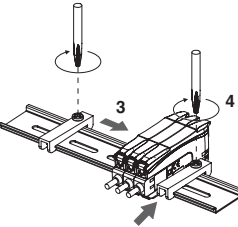
Tighten the screw while pressing the End Plate.
