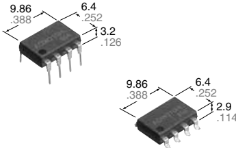
mm inch
