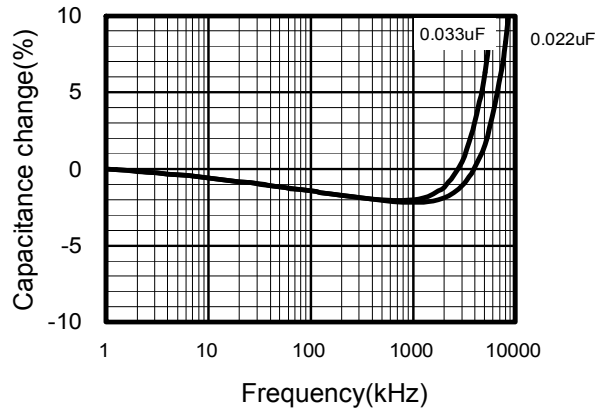
Frequency Characteristics
