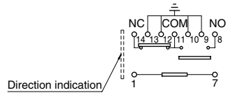
(Deenergized condition)
