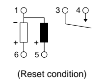
2 coil latching type
