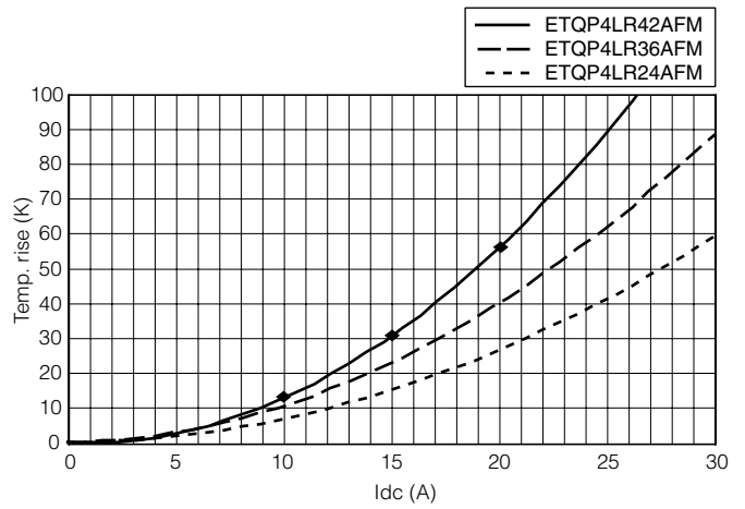
Case Temperature vs DC Current
