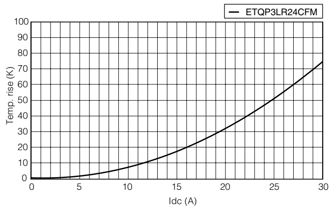
Case Temperature vs DC Current
