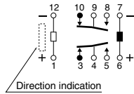
(Reset condition)
