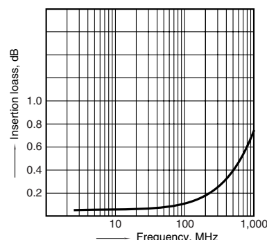
11.-(2) High-frequency characteristics Insertion loss characteristics
