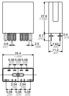
External dimensions
