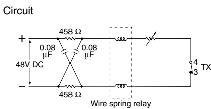
11. Pulse dialing test Tested sample: TX2-5V, 6 pcs. (35 mA 48 V DC wire spring relay load)
