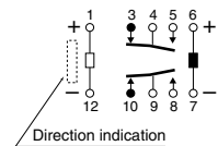
Schematic (Bottom view) 2 coil latching
