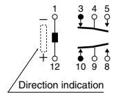
1 coil latching
