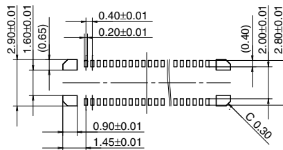
Recommended metal mask pattern Metal mask thickness: When 120μm (Terminal opening ratio: 70%) (Metal-part opening ratio: 70%)
