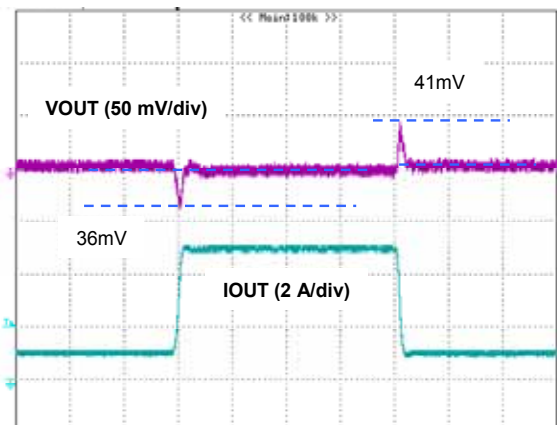
Time (100 \mu\text{s}/\text{div} )
