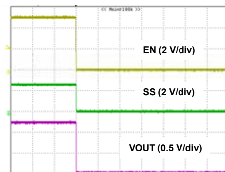
Time (10 ms/div)
