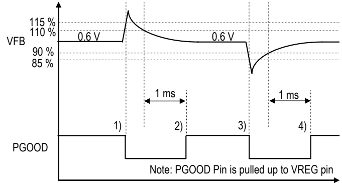
Figure : OVD and UVD Operation
