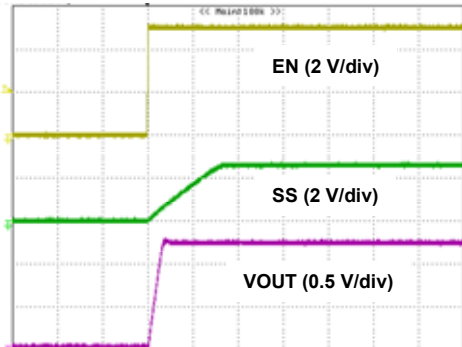
Time (10 ms/div)
