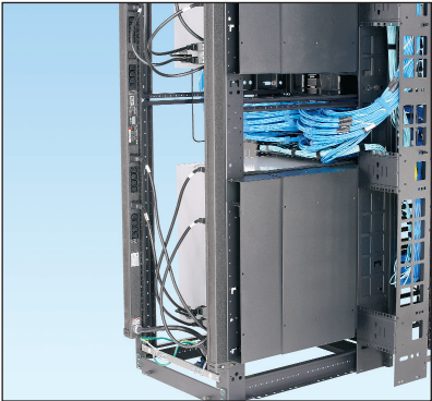
Panduit 4 post rack thermal ducts shown in a dual Nexus 7009 switch deployment.
