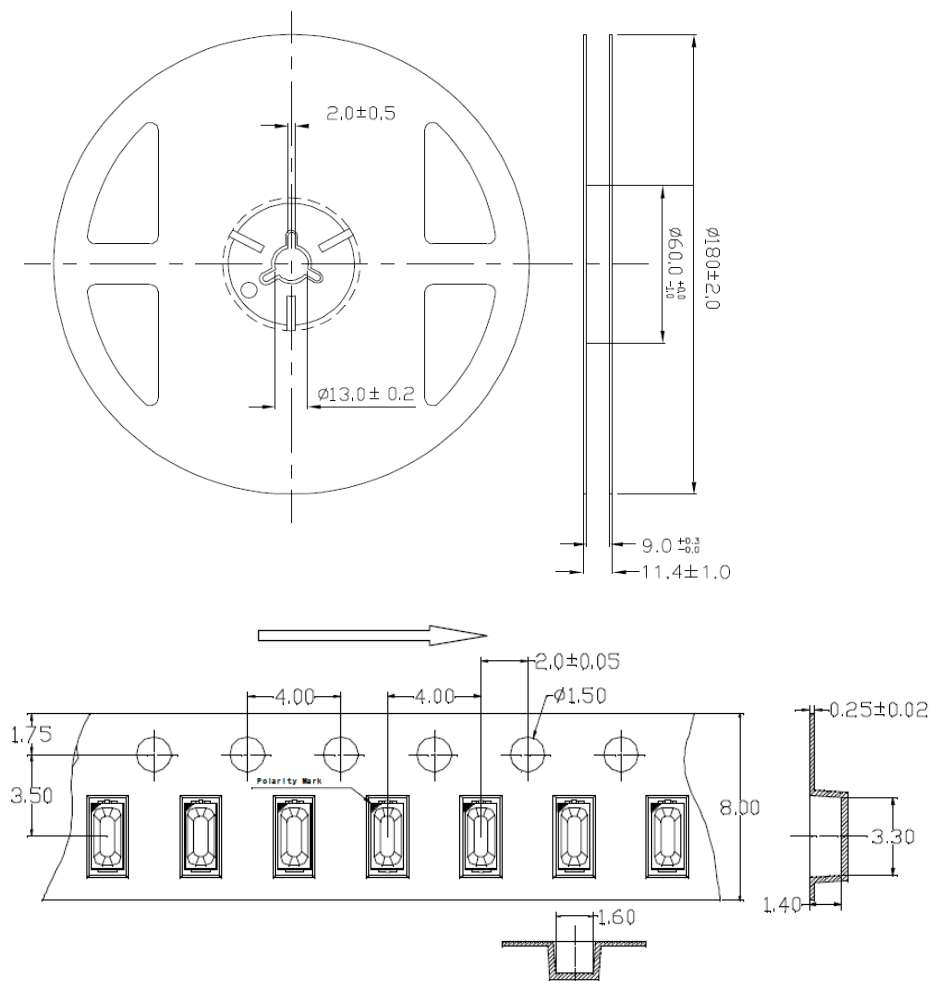
Figure 12. Reel specification (unit in mm)
