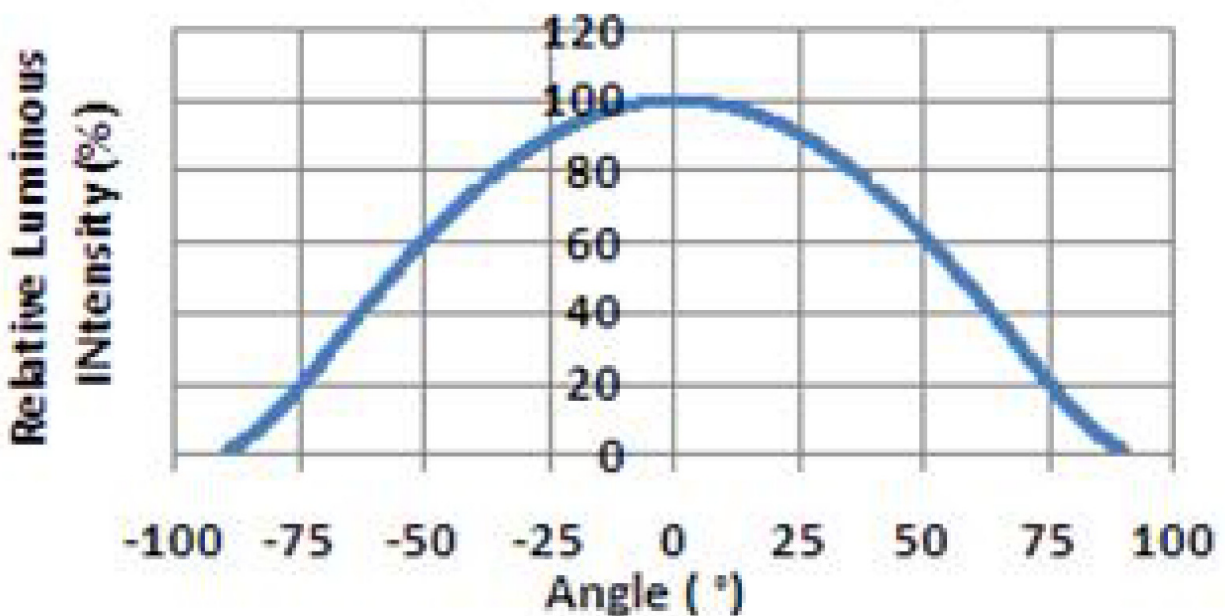
Figure 3. Angular distribution pattern of emitted light
