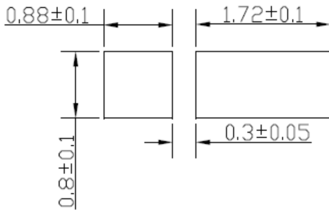
Figure 10. Diagram of soldering pad (unit in mm)
