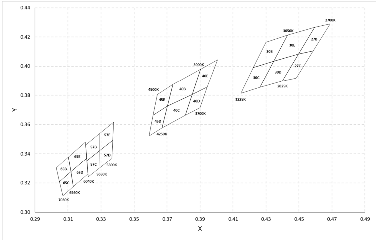
Figure 1. Colour Chromaticity Binning
