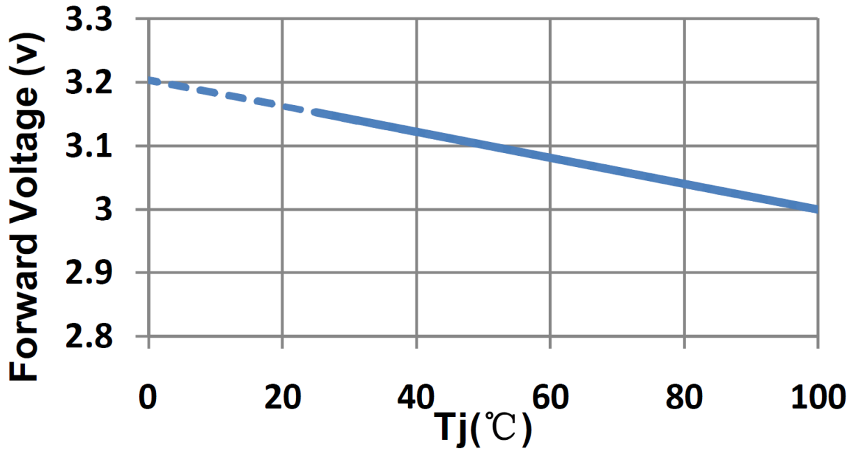
Figure 6. Typical forward voltage versus junction temperature ( I_F=30mA )
