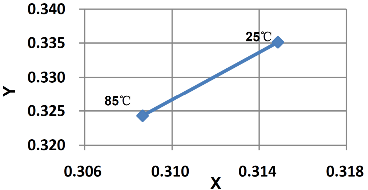
Figure 7. Chromaticity coordinates versus ambient temperature
