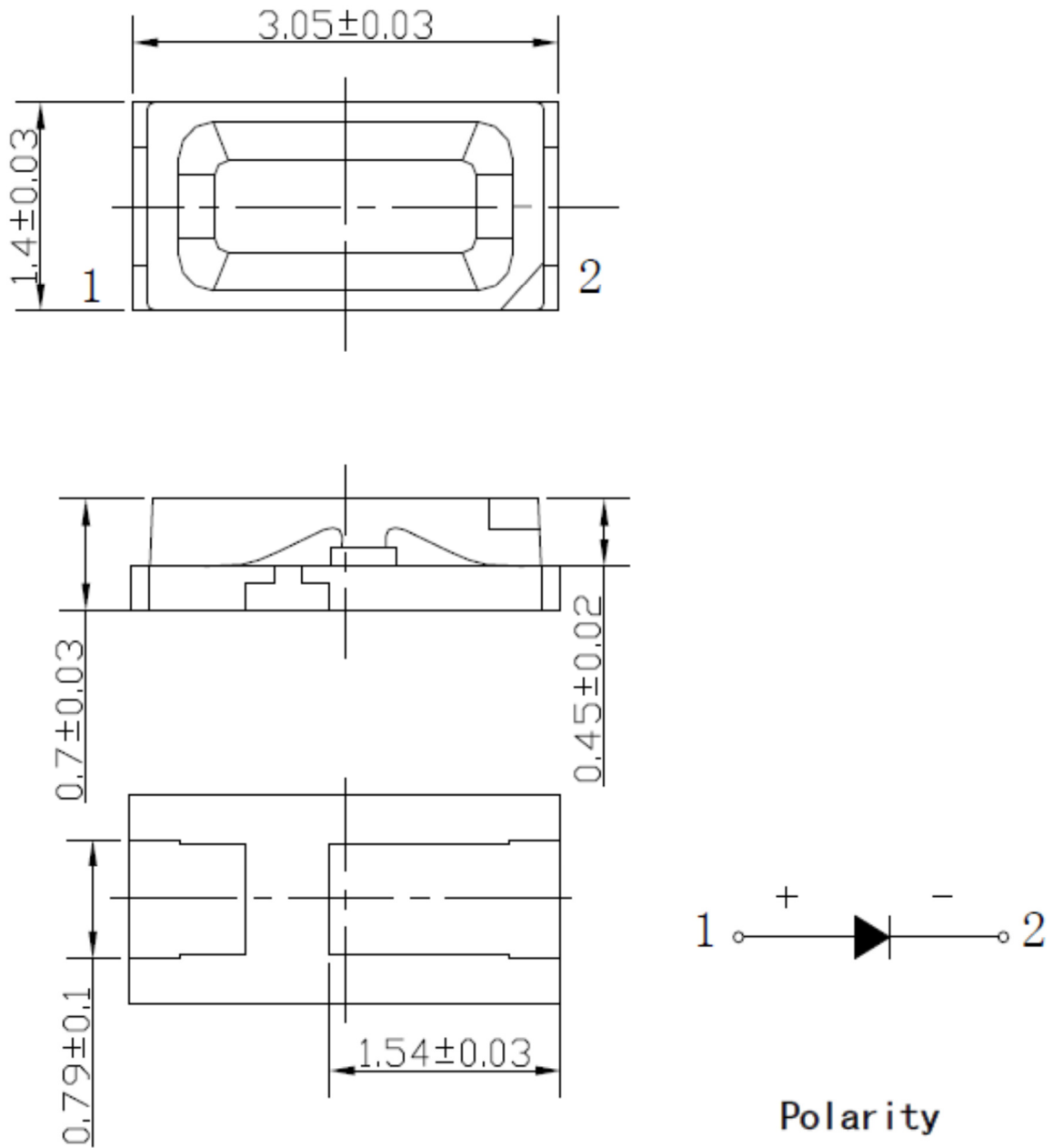
Figure 9. Mechanical drawings of the 3014 package (unit in mm)
