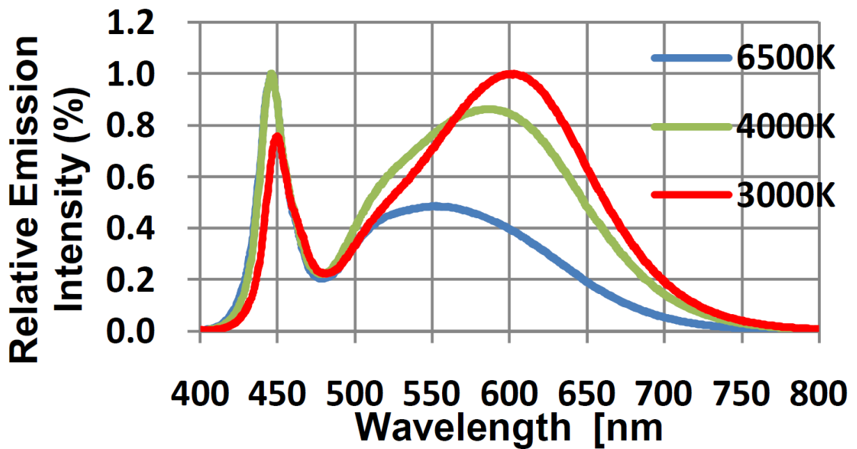
Figure 2. Normalised spectral power distribution (3000K, 4000K & 6500K)
