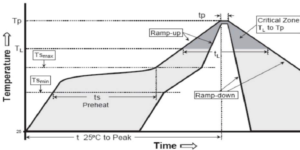
Figure 11. Reflow soldering profile
