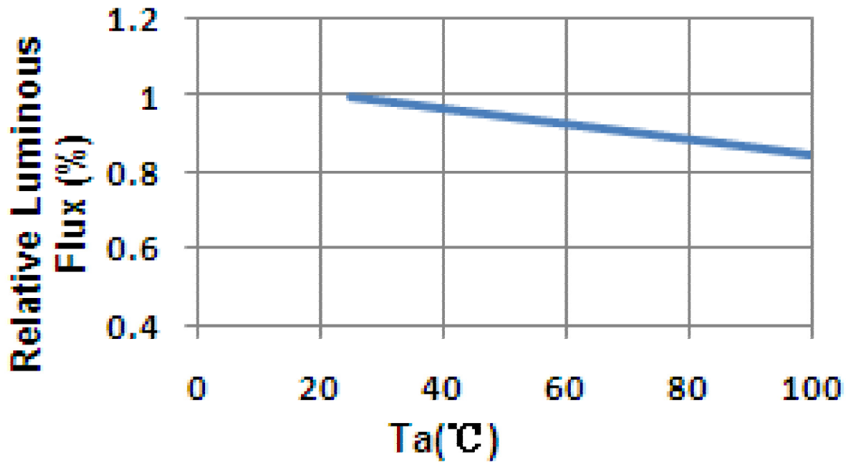
Figure 8. Ambient Temperature vs Relative Intensity
