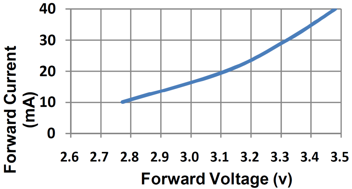
Figure 4. Typical forward current versus forward voltage ( T_a=+25C )
