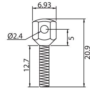
SCREW 4-40, Brass Nickel Plated
