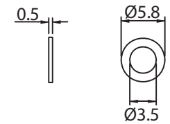
WASHER Brass Nickel Plated
