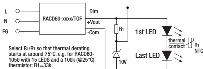
LED Current
