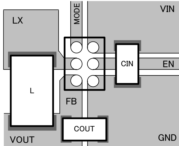
Figure 50. PCB layout
