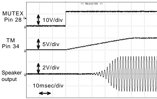
Fig. 13 Wave form when Releasing Soft-mute
