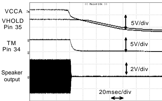
Fig. 15 Wave form on Instantaneous Power Interruption(20msec / div)
