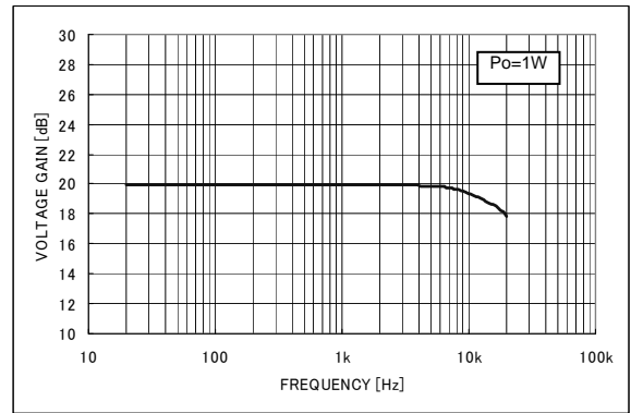
Fig.20 Voltage gain - Frequency
