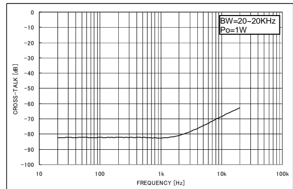
Fig.24 Crosstalk - Frequency
