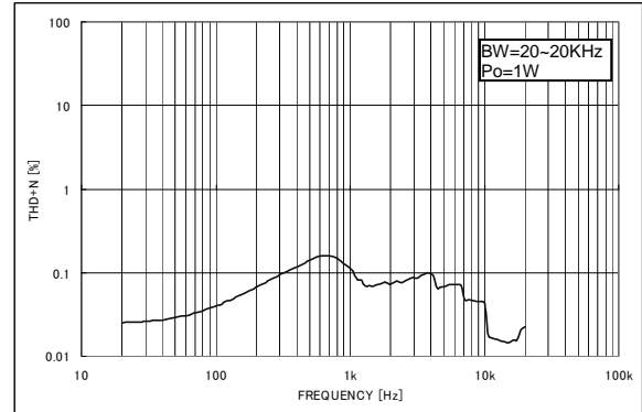
Fig.22 THD+N - Frequency
